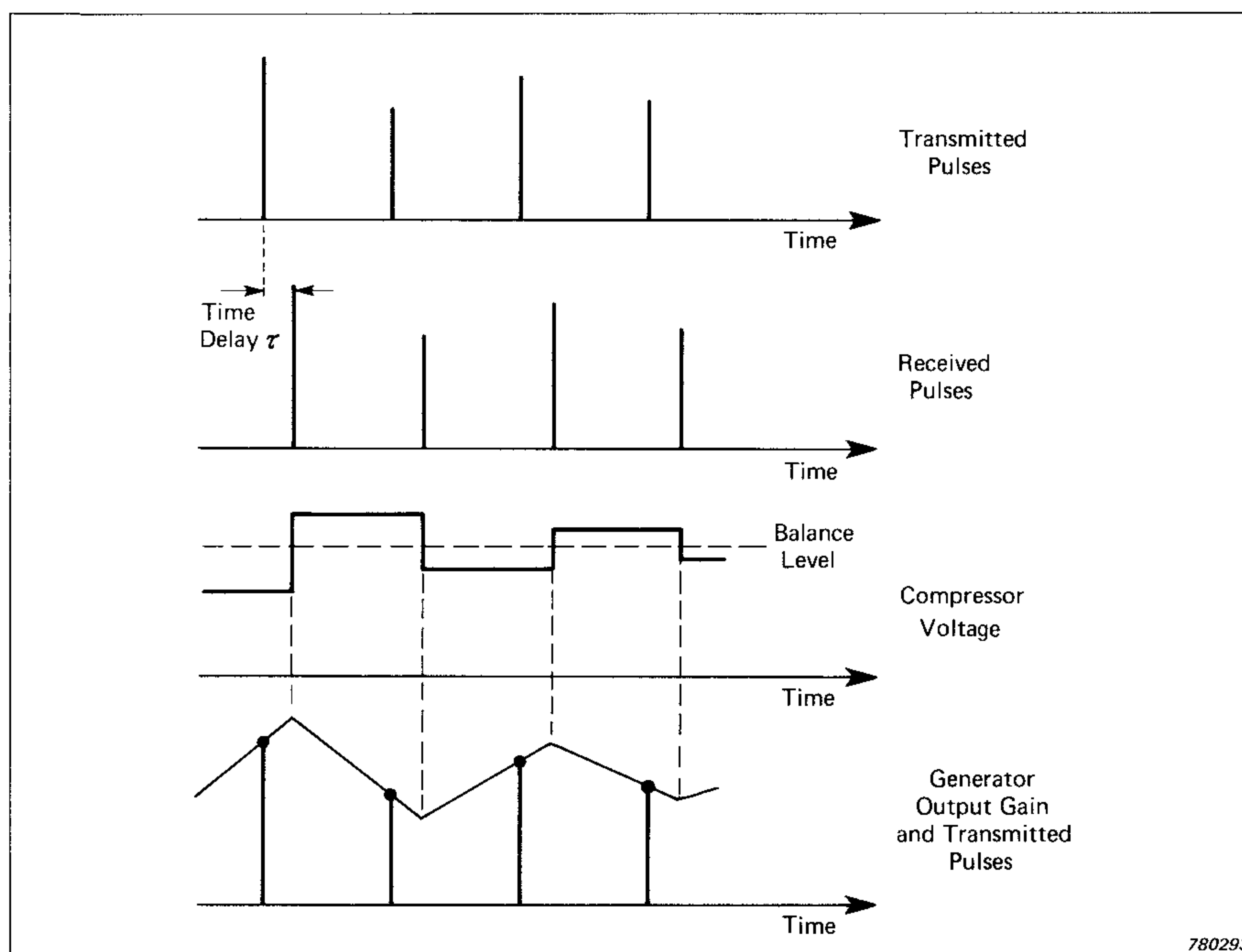
Fig.B1. Influence of time delay
