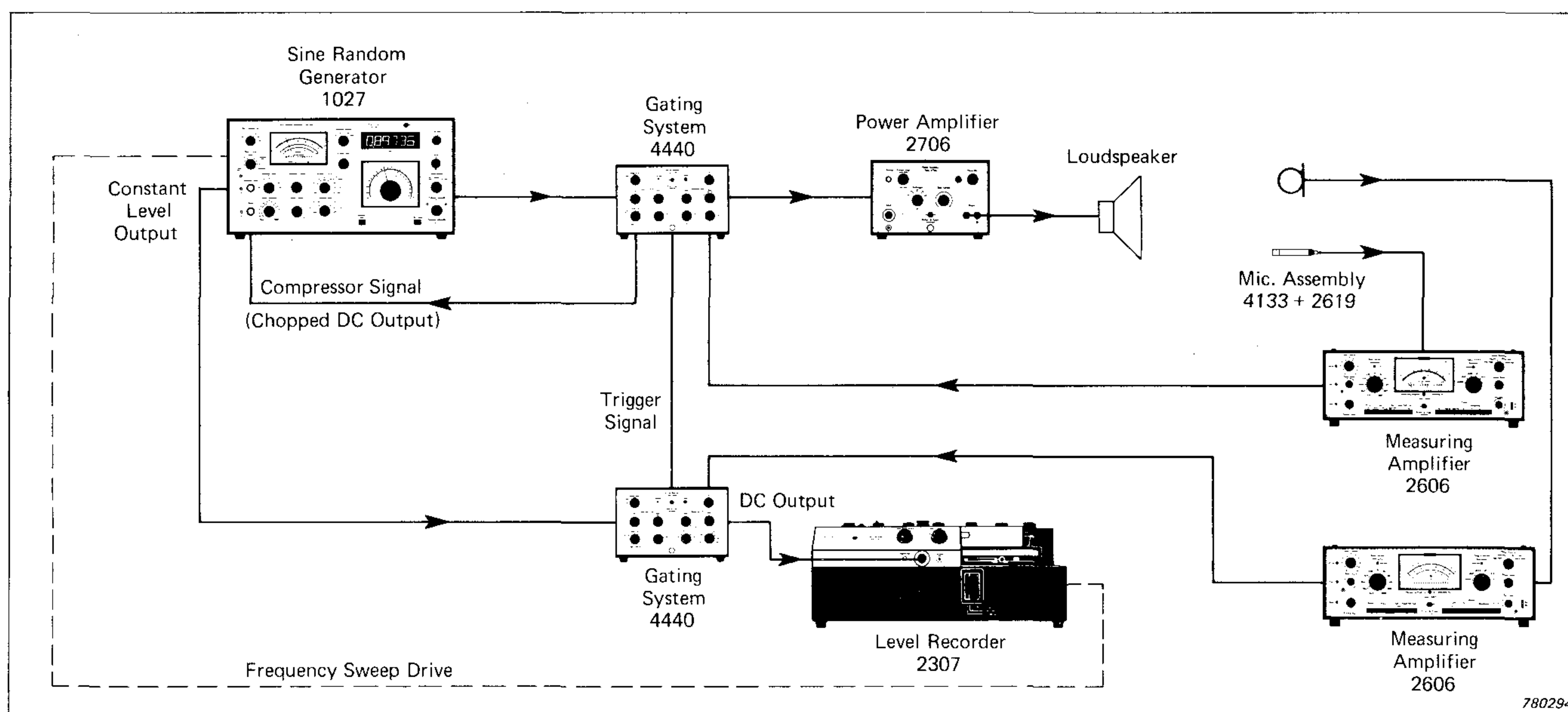
Fig.8. Typical set-up for microphone measurements
