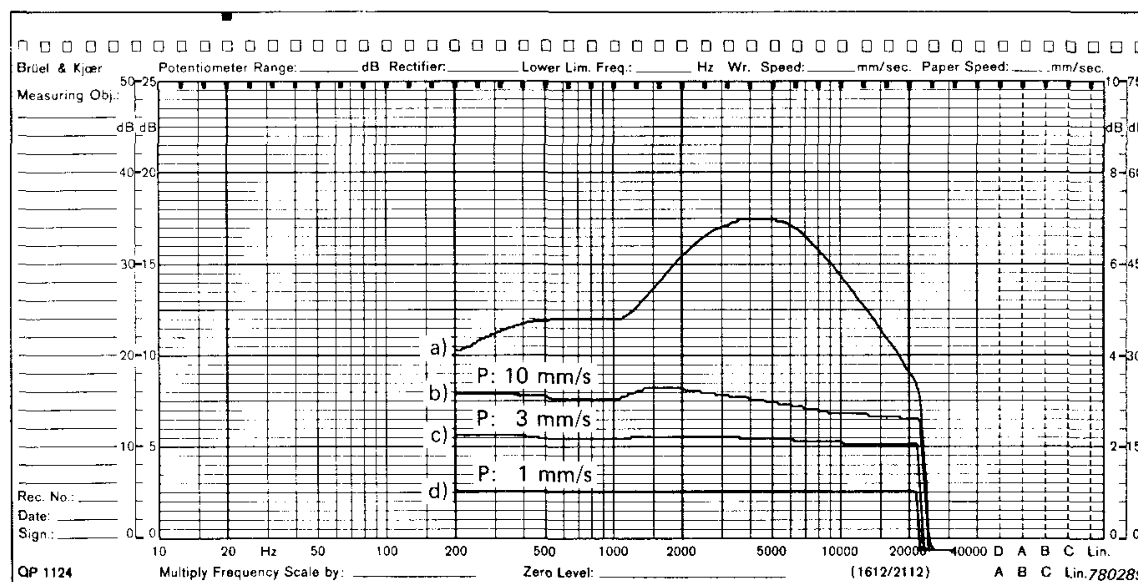
Fig.7. Influence of sweep speed
